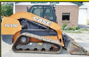
2019 CASE TV370: 1,858 Hours, 3700 Lb Lift, Hyd Coupler, Cab W/ A/C, 2 Speed, Joystick Controls, 78" Bucket, Turbo, 9.7k Lbs, stk#SK967, $39,500
