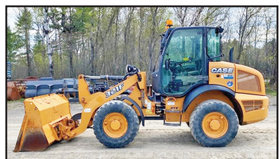
2015 CASE 321F WHEEL LOADER. 1,453 Hours, AC, Heat, Enclosed ROPS, Coupler, Quick Attach, #EQ0019845, $55,000.
