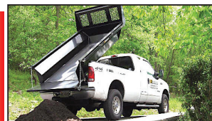
8' Ft & 6 Ft EZ Slide In Dump Body. With Head Board, Tarp & Hoist.
