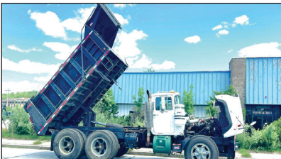
2000 MACK DUMP TRUCK. 350, Allison Automatic, 58K Rears, New 12 X 24 Goodyear Tires, 138K Original Miles, Loaded, Price $42,500. Call For More Information.
