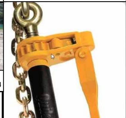
LOCKABLE, FAST, FOLDING HANDLE 670-680 This Chain Tensioner Is Twice As Fast As A Regular Tensioner, Has A Folding Handle For Ease Of Storage, And Can Be Locked With A Padlock For Additional Load Security. 12,000 LB WLL. 888-611-8277
