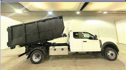
2026 F550 ROLL OFF. Super Cab, Switch N Go, 7.3L Gas, 4WD, Tool Box, Remote Start, Pwr Onboard, F214579. MSRP $114,990. SAVE $11,000. SALE PRICE $103,990
