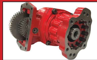
Hot Shift Power Take Offs For Allison
