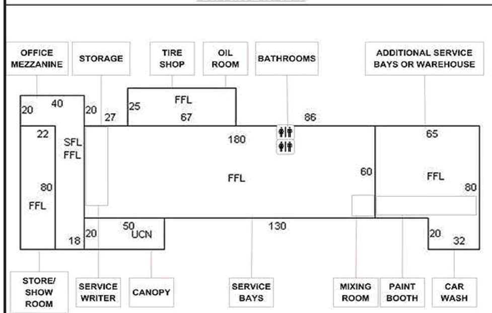
BUILDING SKETCH
